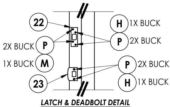
LATCH & DEADBOLT DETAIL
