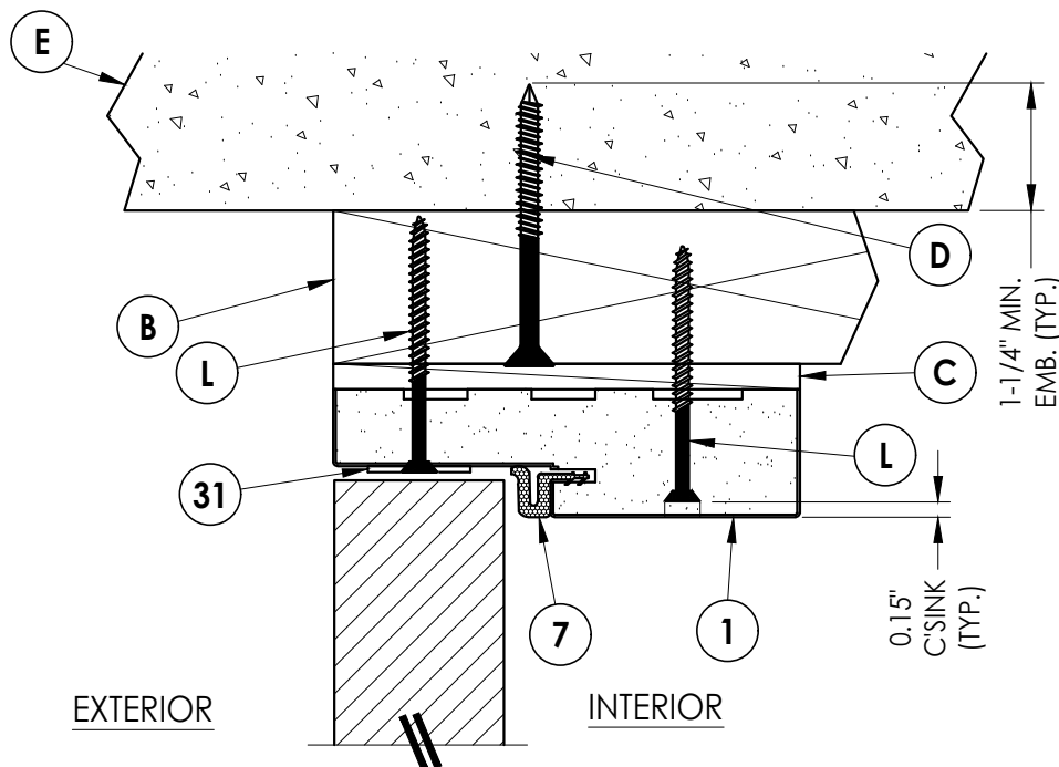
2 4 VERTICAL CROSS SECTION 2X Buck Construction- Double door Outswing shown (Inswing Similar)
